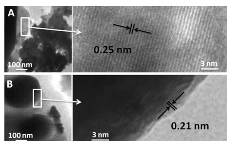
Figure 2. TEM images: A) cobalt monoxide (CoO) and B) cobalt metal prepared by pyrolysis of iodide-paired cobaltocenium-containing polyelectrolytes under air and a \text{H}_2/\text{N}_2 atmosphere, respectively, at 800^\circ\text{C} . On the right are HR-TEM images.
